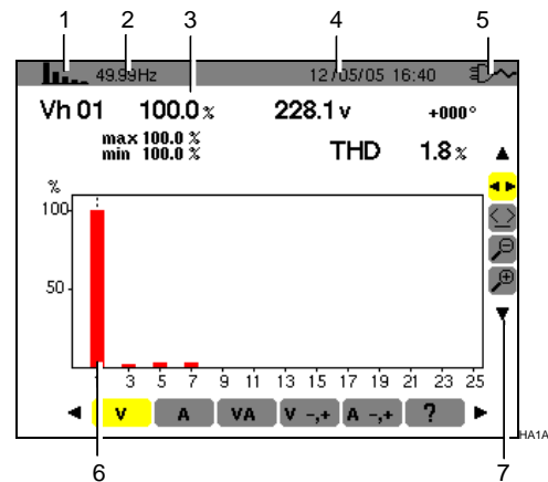
Figure 36: Example of display of harmonics of the voltage.
